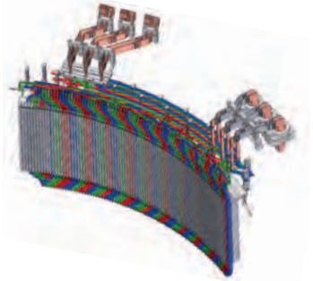
Computerized design tools allowed modeling of the performance of the Smith Mountain generator.
